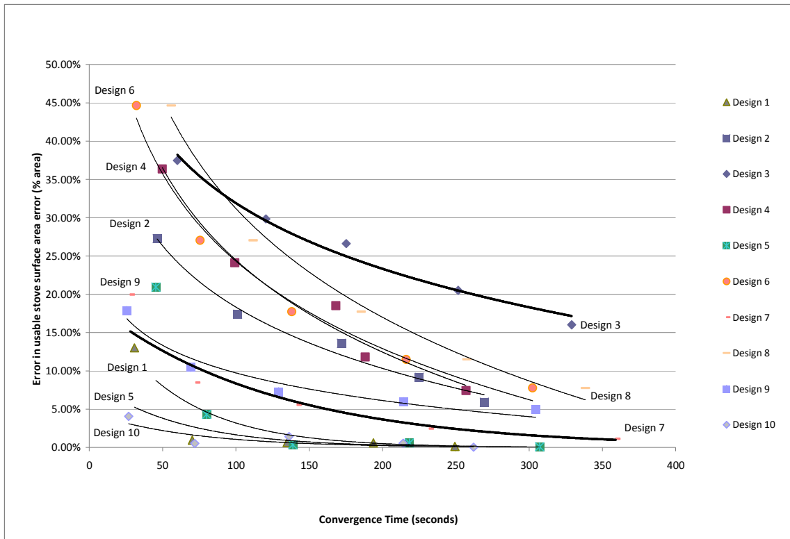
Figure 71 - A_{\text{error}} usable area values for grids of fixed plane resolution
